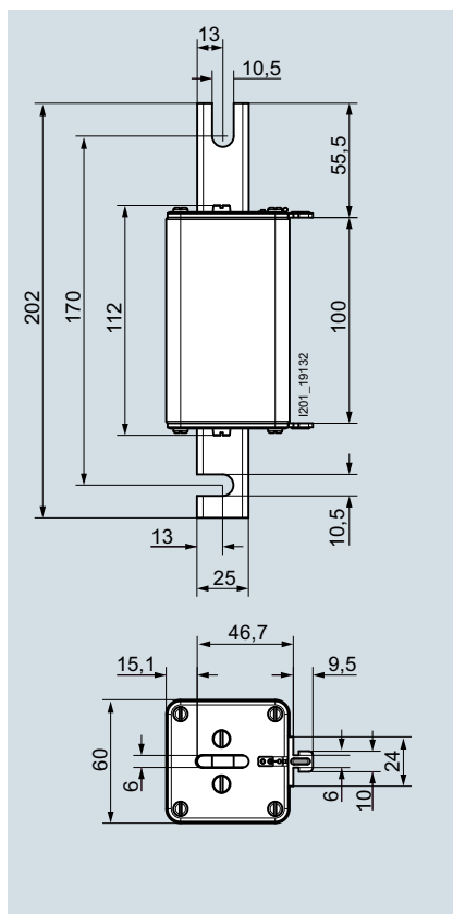
3NB1231-4KK11 3NB1234-4KK11
