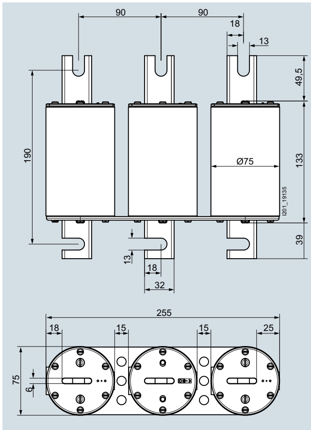
3NB2364-4KK17, 3NB2366-4KK17
