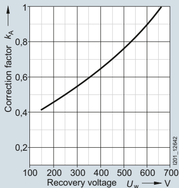
Correction factor k_A for breaking I^2t value Example: Series 3NE8 0..
