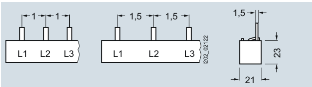
5ST3710-0HG 5ST3714-0HG
