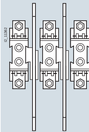
3 LV HRC fuse bases, 1P
