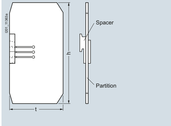
LV HRC partition
