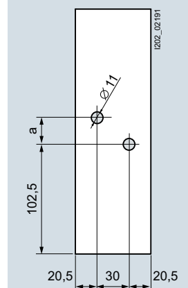
Drilling plan
