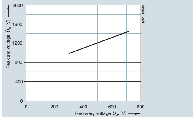
Peak arc voltage
