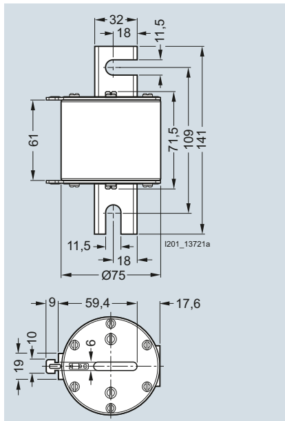
3NC24...-3C, 3NC84...-3C
