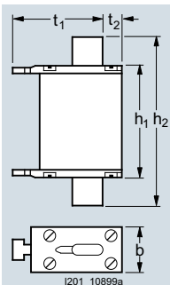
Size 4 (IEC design)
