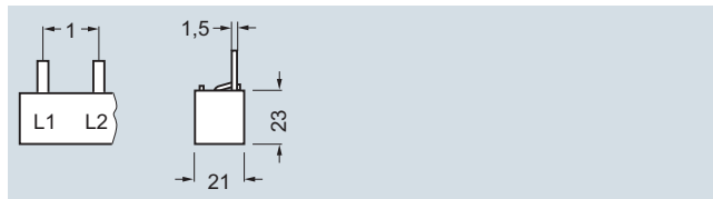
5ST3705-0HG
