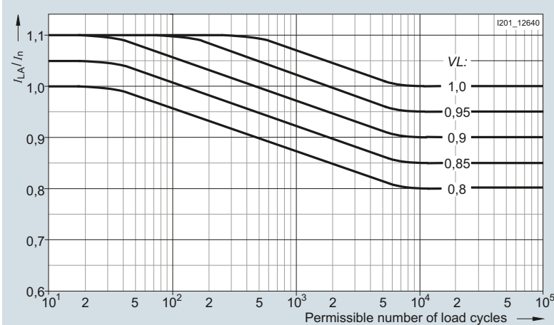
Waveform of the varying load factor VL for load cycles
