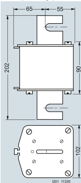
Size 4 (IEC design)
