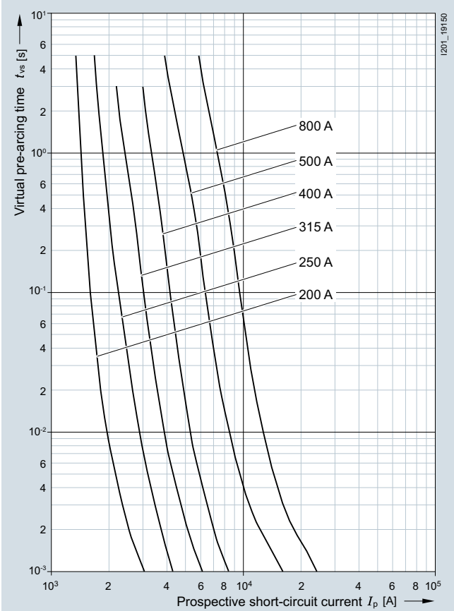
3NB1...-4KK11
