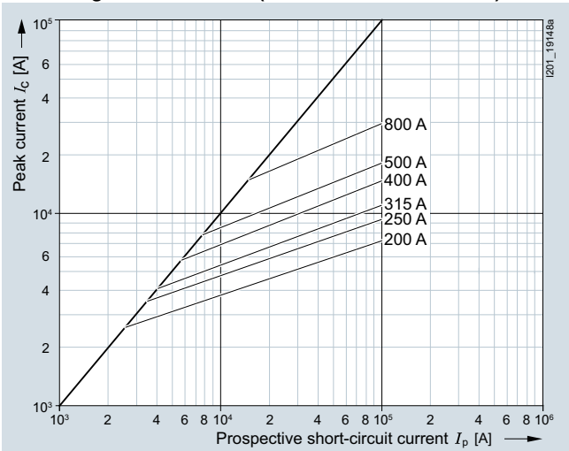
3NB1...-4KK11
