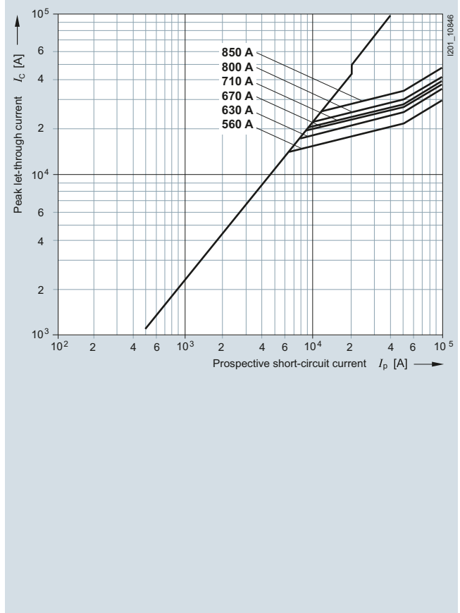
Let-through characteristics (current limitation at 50 Hz)
