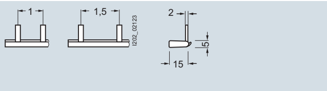
5ST3701-0HG 5ST3703-0HG
