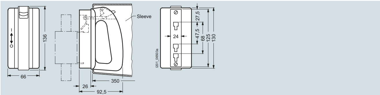
3NX1013 (without sleeve), 3NX1014 (with sleeve)
