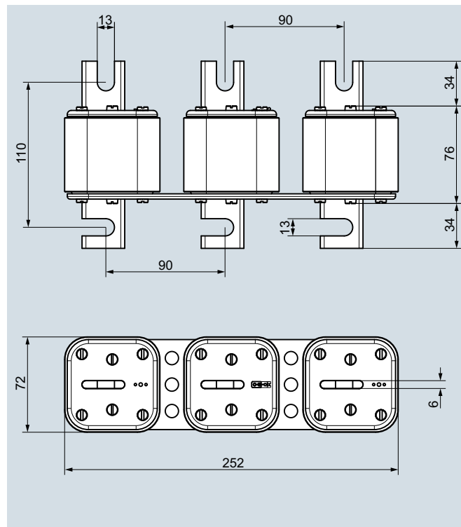
3NB3358-1KK27 3NB3362-1KK27
