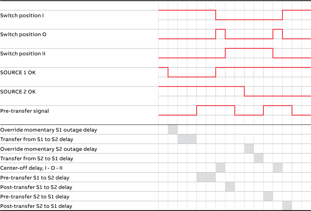
No source priority (generator and load shed usage disabled)
