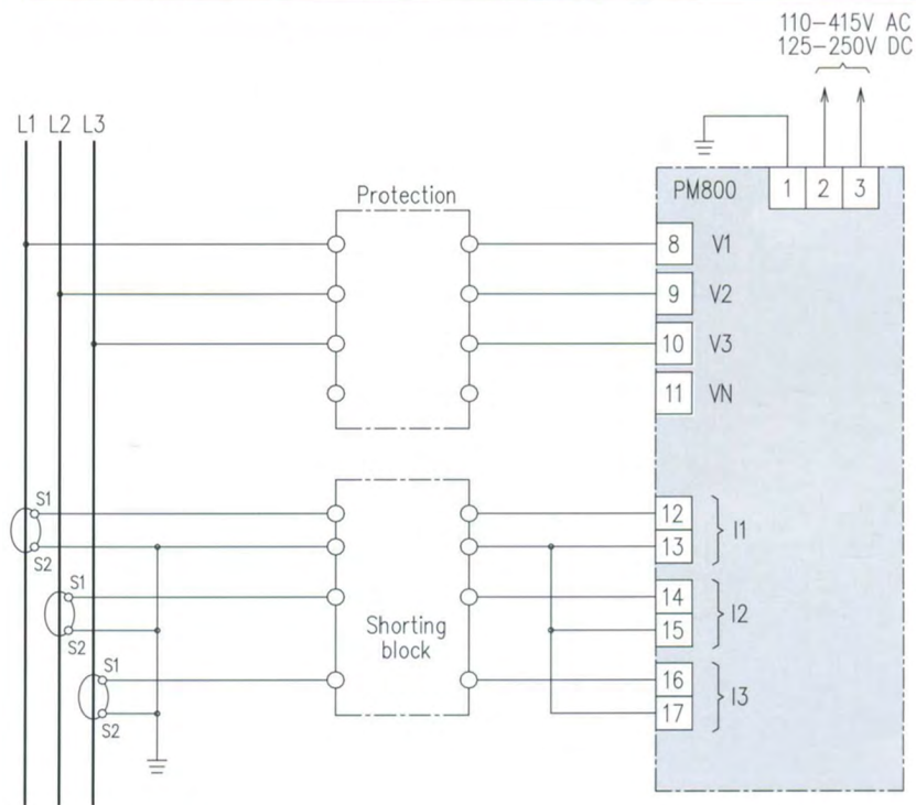
Connection example.
