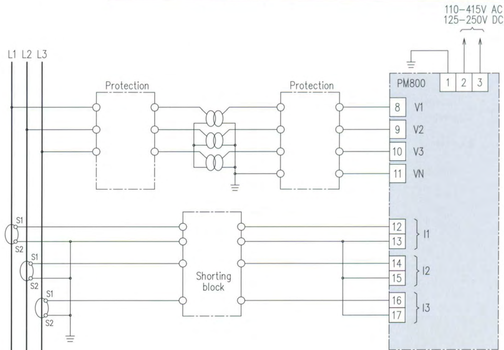
Connection example.
